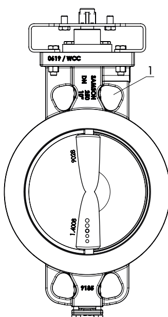
Fig. 3b: DN 150 to 400/ NPS 6 to 16
