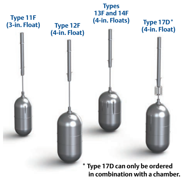
Figure 2. Float element types
