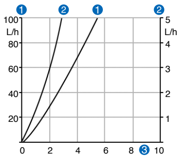
杆Φ1.0mm
