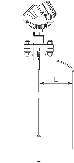
Figure 22: Free Space Requirement
