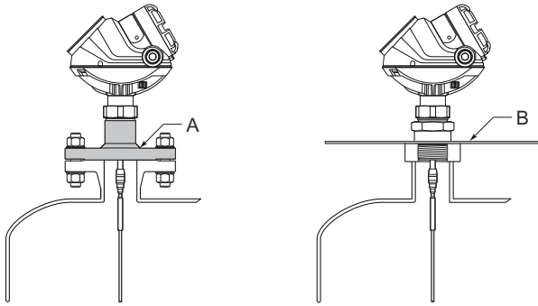
Figure 27: Mounting in Non-Metallic Tanks
