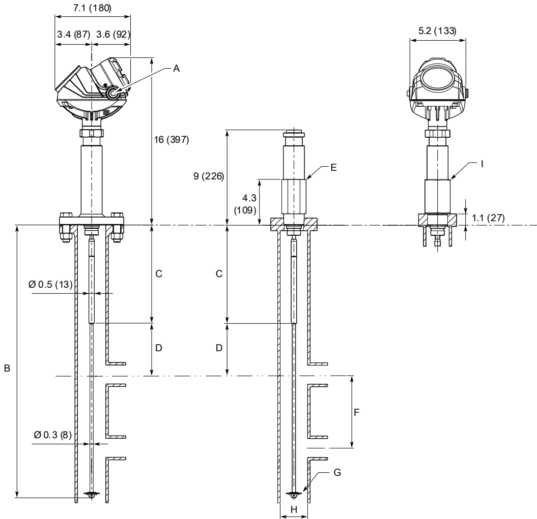
Figure 36: Single Rigid Vapor Probe for 2-in. Chambers
