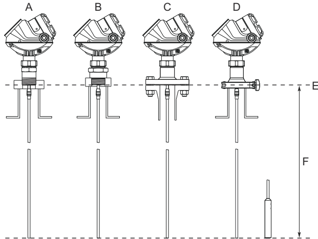
Figure 21: Total Probe Length
