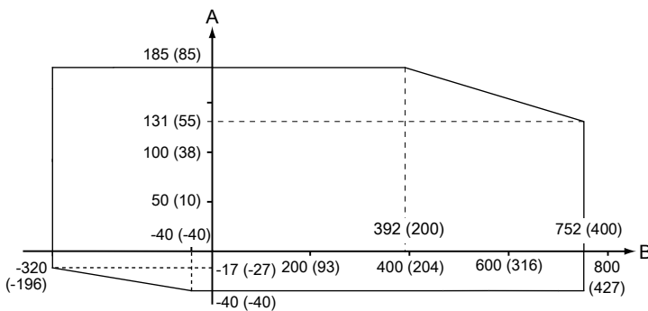
Figure 15: Ambient Temperature vs. Process Temperature
