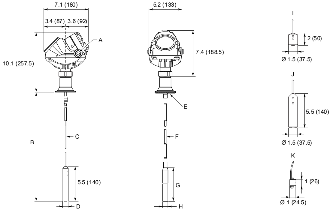
Figure 38: Flexible Single Lead Probe with Tri-Clamp Connection
