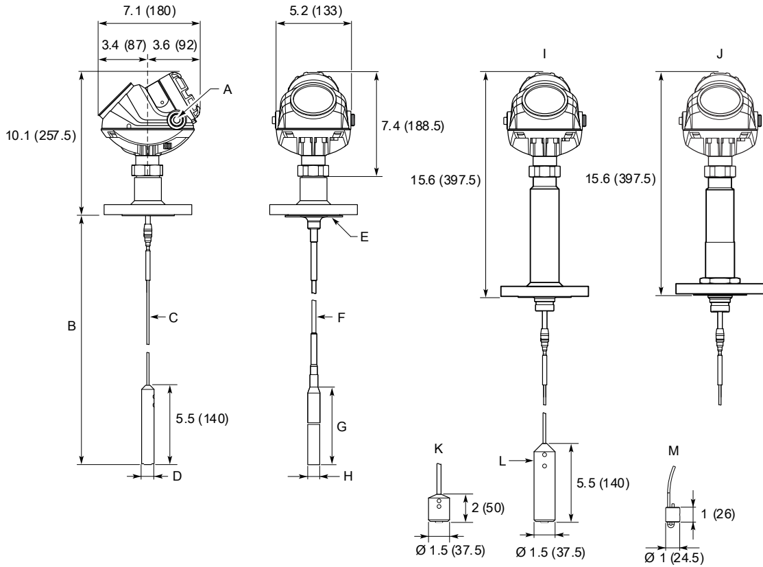
Figure 37: Flexible Single Lead Probe with Flange Connection
