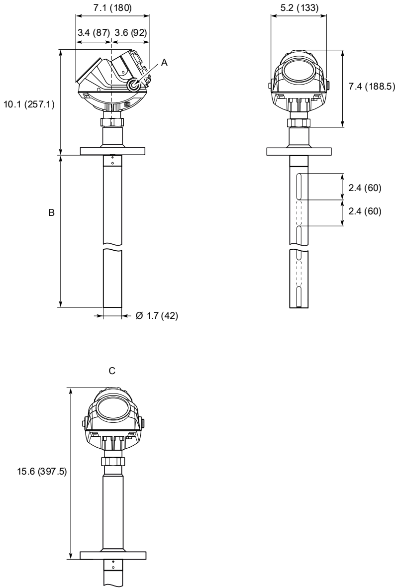
Figure 42: Large Coaxial Probe with Flange Connection
