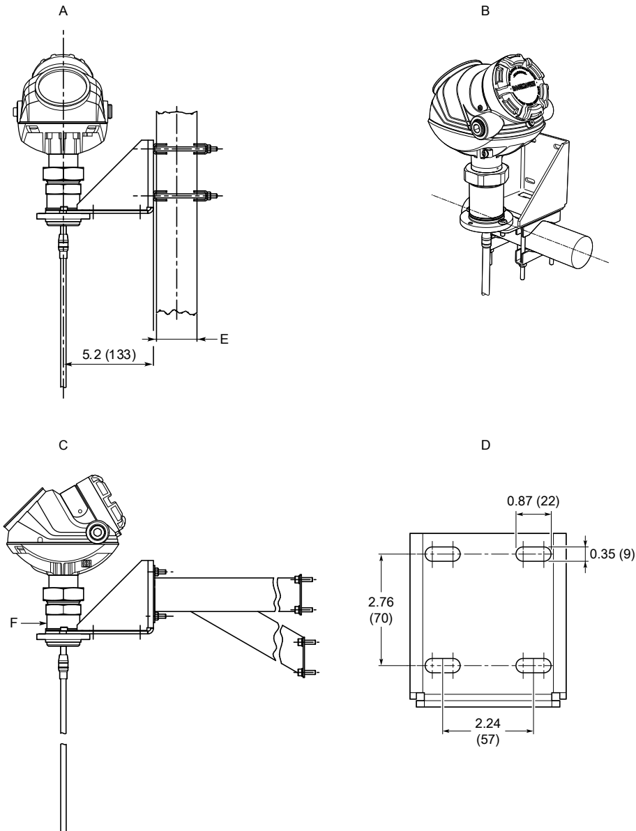
Figure 47: Mounting Bracket (Option Code BR)
