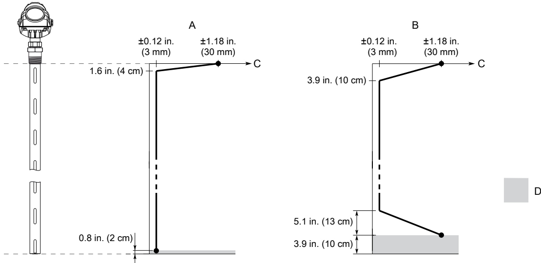
Figure 8: Accuracy Over Measuring Range for Large Coaxial Probe
