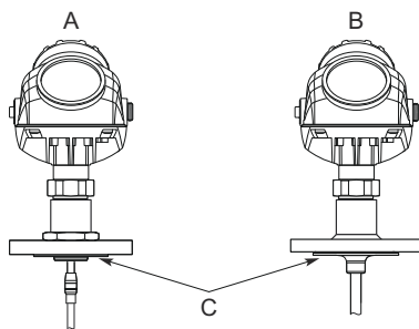
Figure 17: Protective Plate
