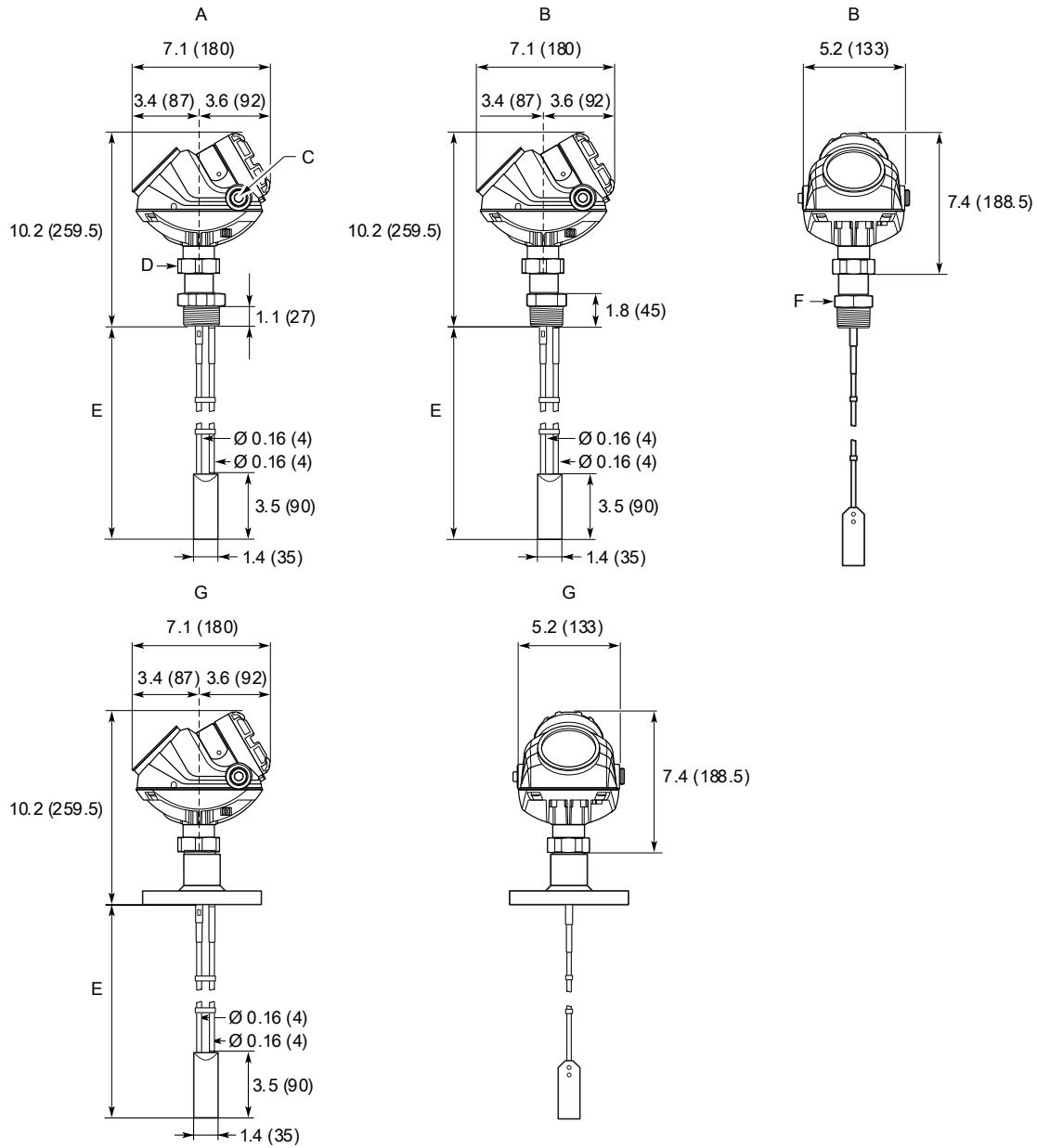
Figure 46: Flexible Twin Lead Probe
