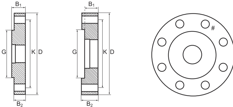
Figure 49: Proprietary Flanges
