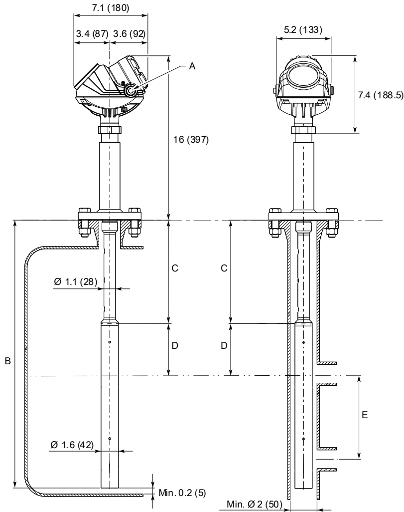
Figure 44: Integrated Still Pipe Vapor Probe for 3-in. Chambers and above
