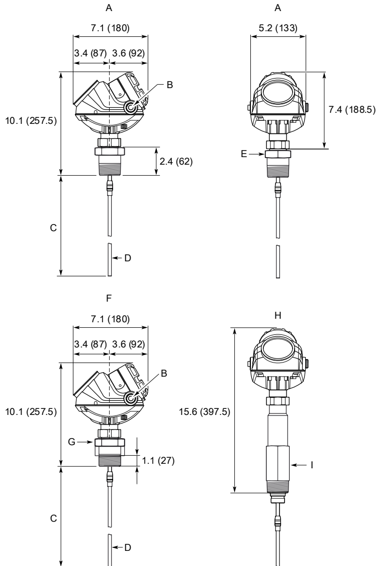
Figure 33: Rigid Single Lead with Threaded Connection
