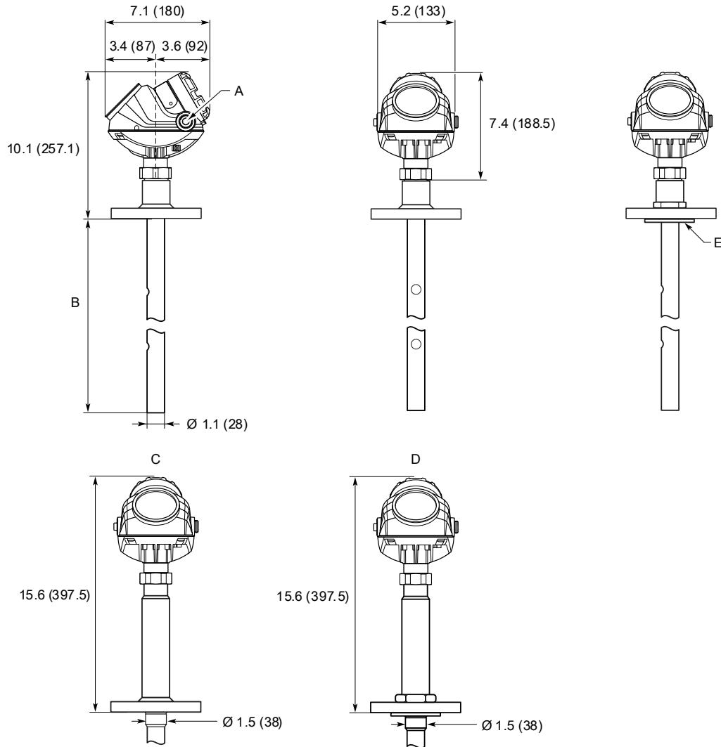
Figure 40: Coaxial probe with Flange Connection
