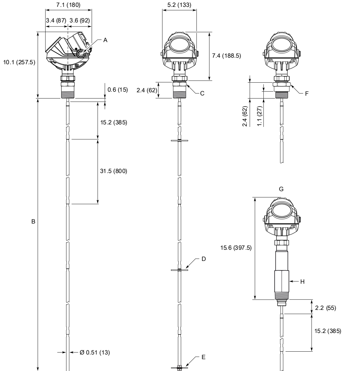
Figure 35: Segmented Rigid Single Lead Probe with Threaded Connection
