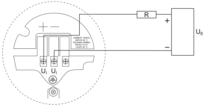
Figure 11: External Power Supply for HART
