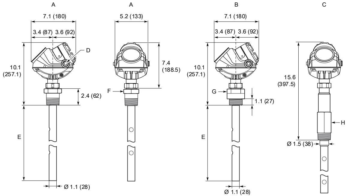
Figure 41: Coaxial Probe with Threaded Connection
