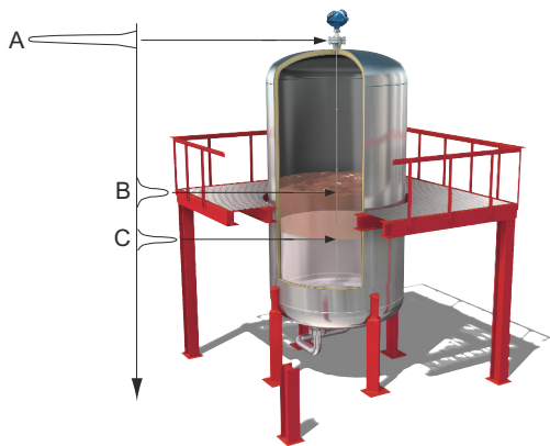
Figure 1: Measurement Principle
