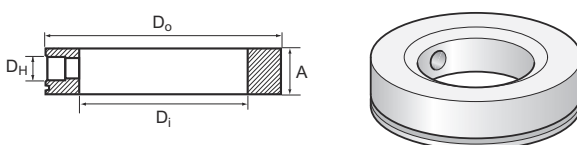
Figure 50: Flushing Connection Rings
