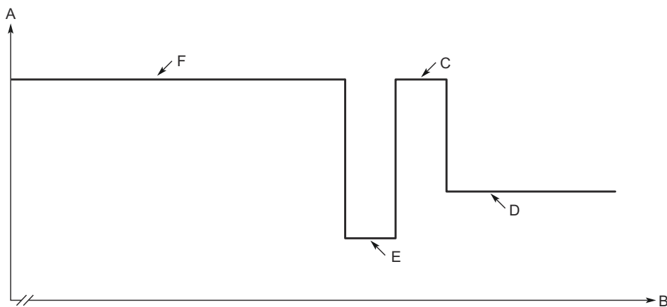
Figure 10: Start-Up Sequence for Option Code BR5 with Ambient Temperatures Below -40 °F (-40 °C)
