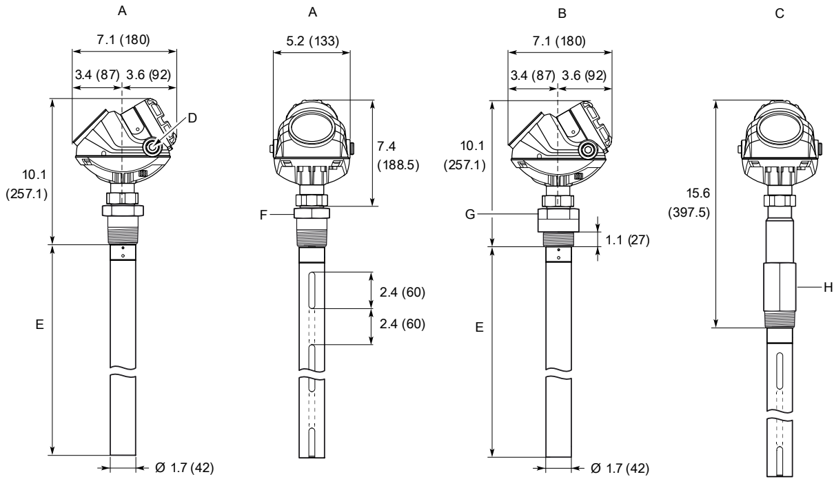
Figure 43: Large Coaxial Probe with Threaded Connection
