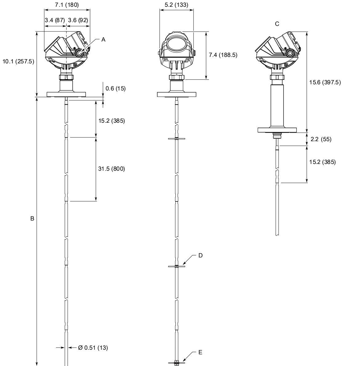
Figure 34: Segmented Rigid Single Lead Probe with Flange Connection
