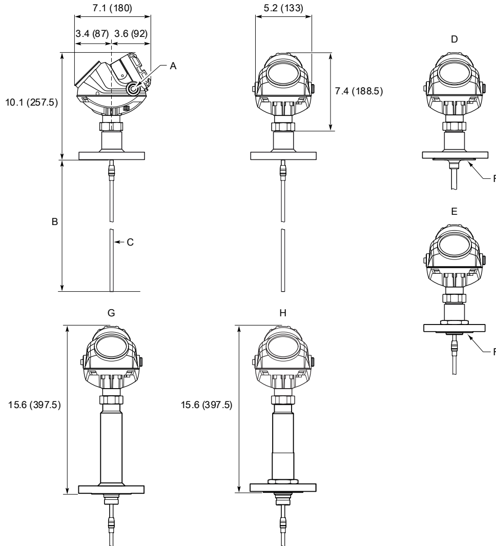
Figure 31: Rigid Single Lead Probe with Flange Connection
