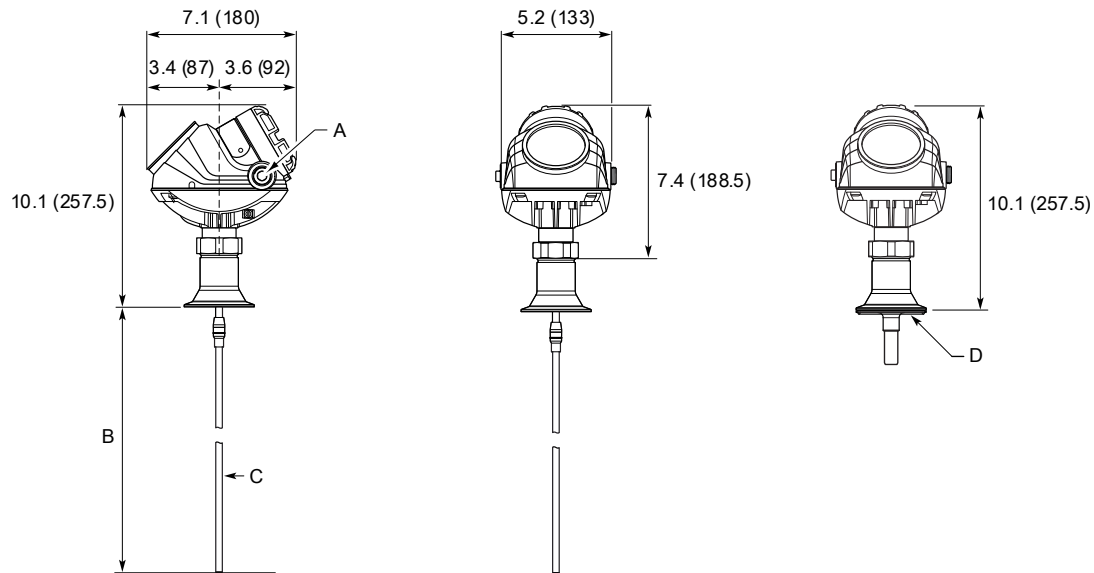
Figure 32: Rigid Single Lead Probe with Tri-Clamp® Connection
