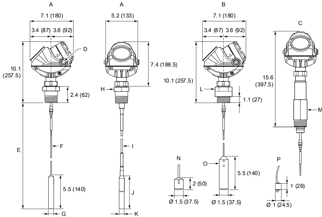
Figure 39: Flexible Single Lead with Threaded Connection
