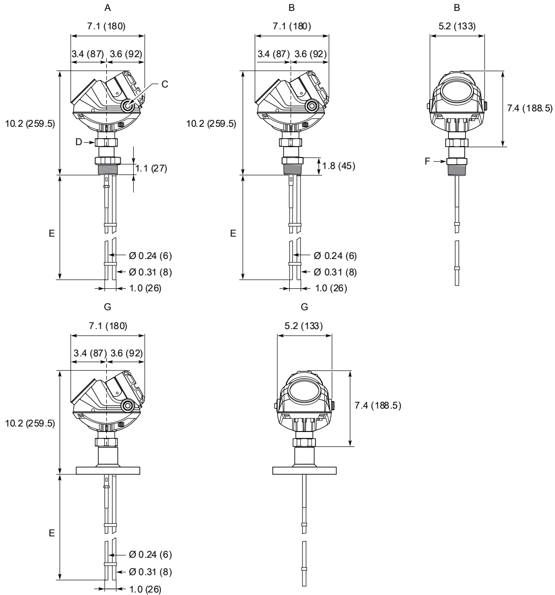
Figure 45: Rigid Twin Lead Probe
