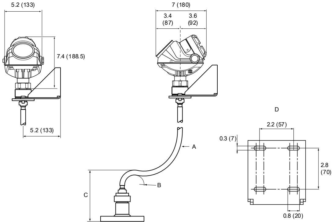
Figure 48: Remote Housing (Option Code B1, B2, B3)
