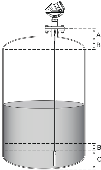
Figure 4: Blind Zones
